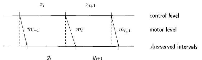
FIG. 7. Schematic illustration of two-level timing. The motor delays are uncorrelated. Due to the measurement procedure, the successive intervals are negatively correlated.
