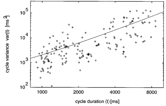
FIG. 6. Relation between cycle variance \text{var}(t) and mean cycle duration \langle t \rangle for subject C. As a rough approximation we obtain a polynomial of second order (18) with a = 1.003 and b = 1.06 \times 10^{-3} . Note that the time series consists of only 12 values, which contributes to the scattering of data points around the regression line.
