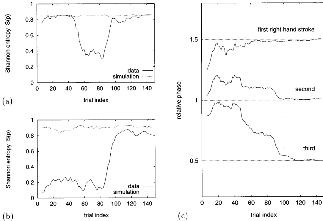
FIG. 3. Shannon entropy (5) of the distribution of words obtained from the data of subject A [left hand (a), right hand (b)]. A low value of the S(p) corresponds to highly regular symbol sequences. The dashed line shows the Shannon entropy for simulated data (surrogates) using the variances as in the experimental time series. (c) A plot of the relative phases (in units of \pi ) also indicates the dynamical transitions.
