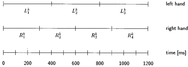
FIG. 1. Schematic illustration of the 3:4 polyrhythmic task used in the study by Krampe et al. [5]; here for a cycle duration of 1200 ms. “R” and “L” in the top panels denote the intervals produced by right and left index fingers, respectively. Each cycle starts with simultaneous strokes of the two hands. Three isochronous intervals, i.e., equidistant strokes in time, in the left hand are performed against four isochronous intervals in the right hand within each cycle. The position of intervals within a certain cycle k is indicated by subindices.
