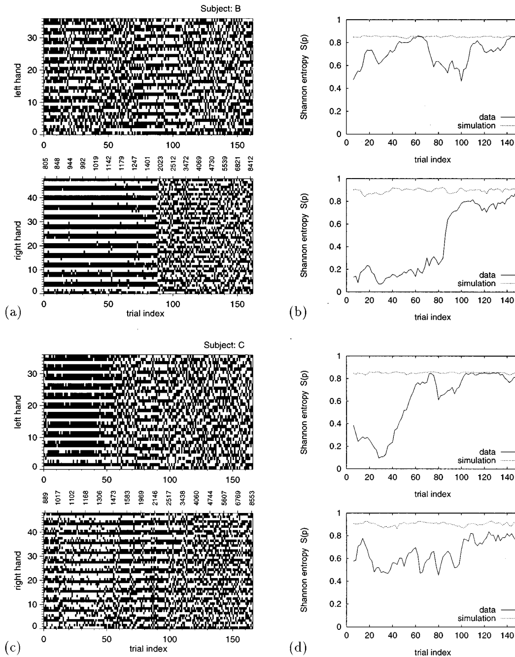
FIG. 4. Symbol sequences of all trials and corresponding Shannon entropies for two other individuals obtained by the two-symbol coding. The data of subject B (a), (b) show a sharp transition in the right hand, whereas the data of subject C (c), (d) are an example for a qualitative transition in the left hand.
