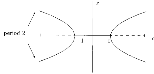
FIG. 5. Bifurcation diagram of the nonlinear error correction model (7). A pitchfork bifurcation occurs at c = +1 . The period-doubling bifurcation ( c = -1 ) creates oscillating solutions for c < -1 which are the basis for reproducing the periodic symbol sequences obtained from the experiments.
