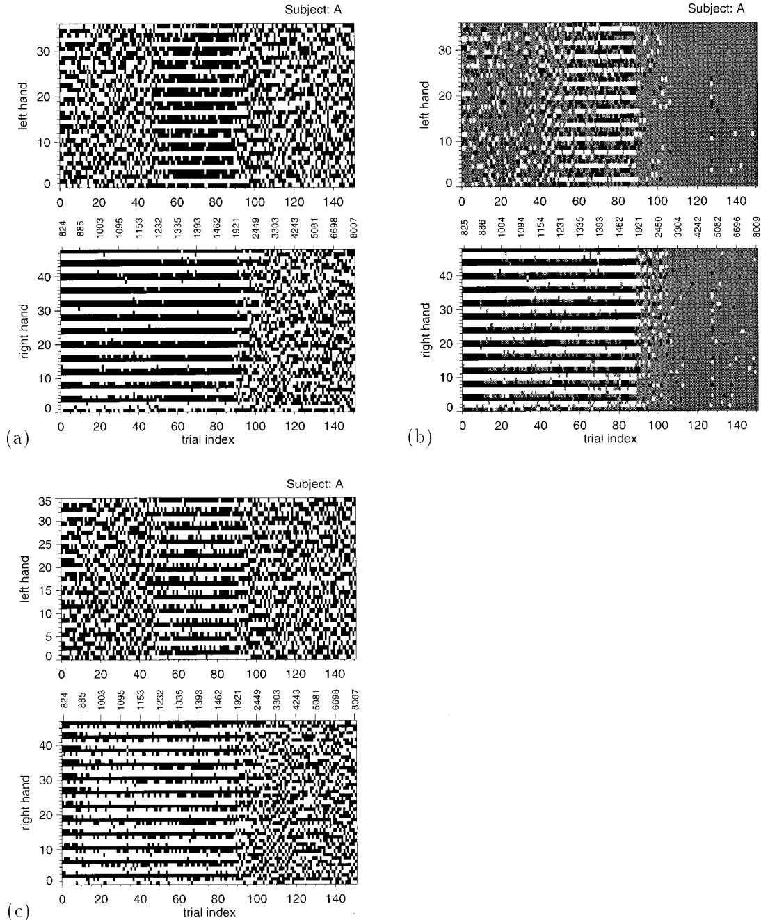
FIG. 2. Symbol sequences of all trials of one individual A. The time is increasing on the ordinate, where 36 symbols are plotted for left hand time series and 48 symbols for the right hand. The trials are sorted with respect to the realized cycle duration. The cycle durations T (ms) are indicated by the vertical labels between the plots. Two-symbol coding (a), defined in Eq. (4), in comparison with three-symbol coding (b). Irregular symbol patterns correspond to accurate performance which is demonstrated by the accumulation of gray symbol in (b). These results are qualitatively stable; the symbol patterns are in good agreement with those obtained by dynamic coding rules (c).
