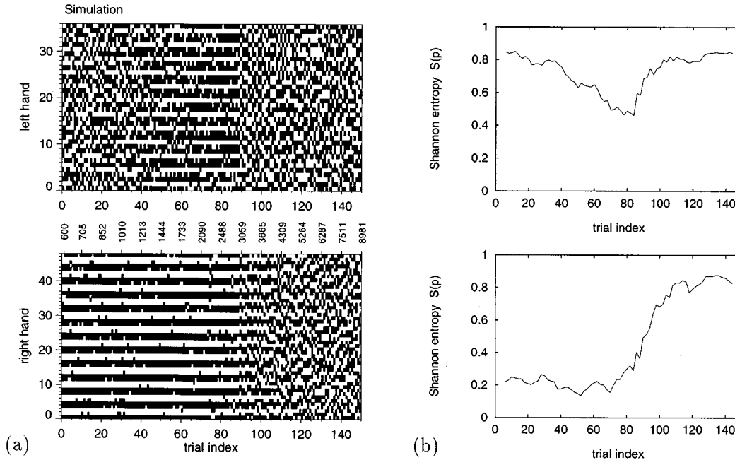
FIG. 9. Example for a simulation of the model in a more complicated case. The symbol patterns (a) and Shannon entropies (b) are qualitatively in agreement with those produced by subject A.
